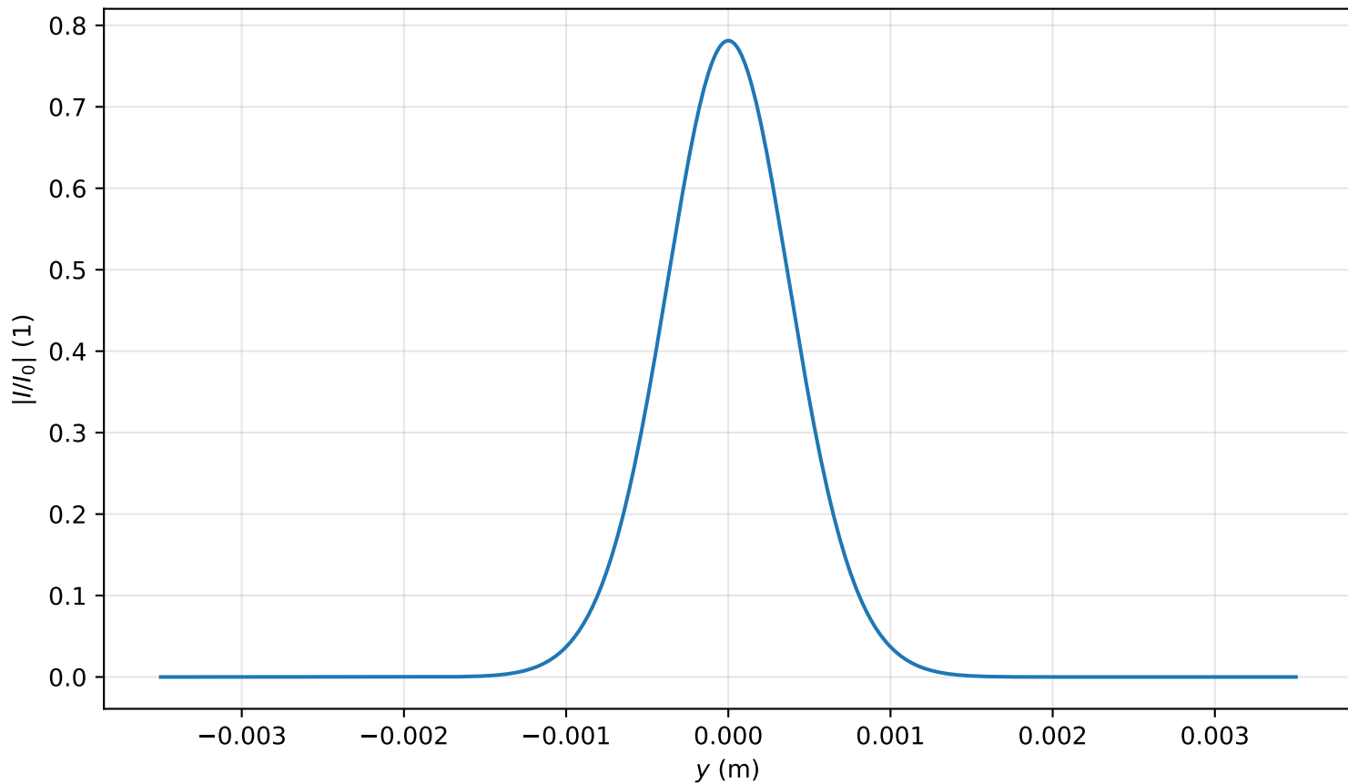
Intensity profile I(x=0, y, z=1.353)/I_0 , P_{in}=0.2P_{cr} , artificial time
